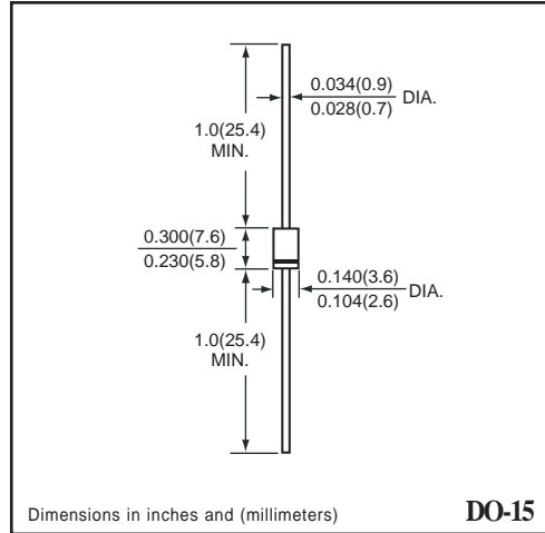
DO-15
